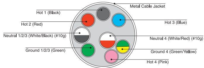
CROSS SECTION 8 WIRE 4 CIRCUIT CABLE
